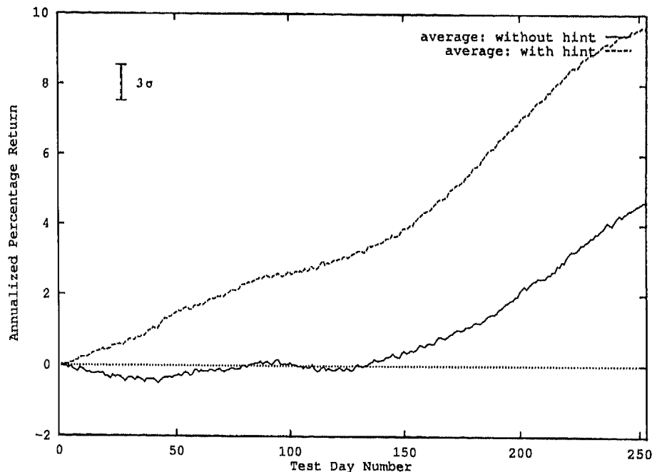
Figure 3. Learning performance with and without hint.
