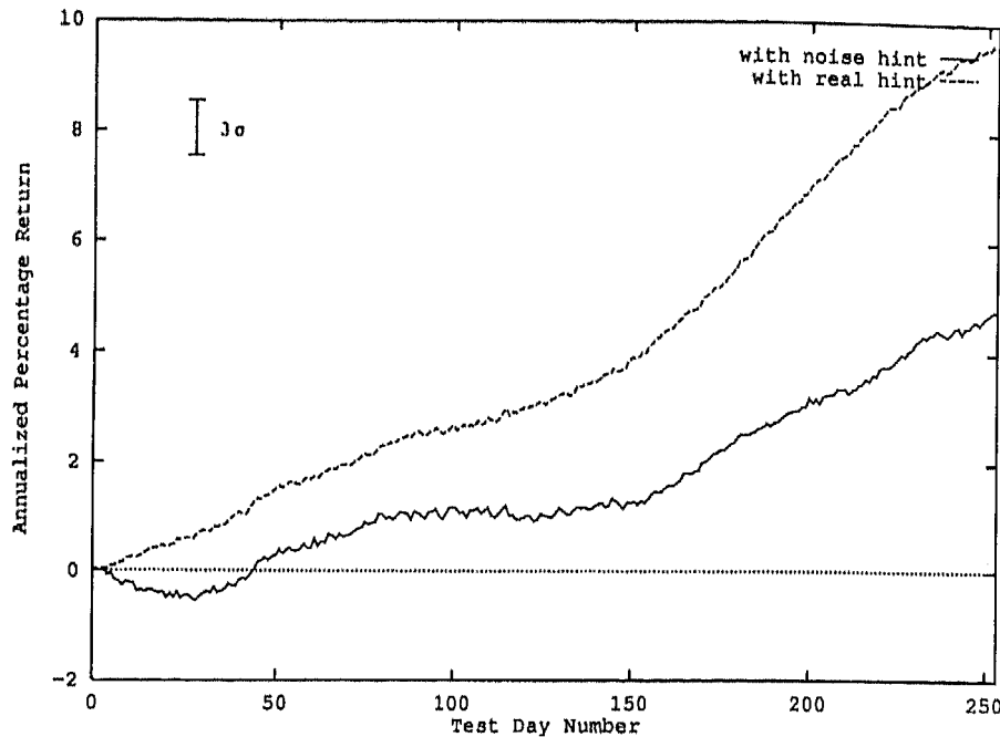
Figure 4. Performance of the real hint versus a noise hint.
