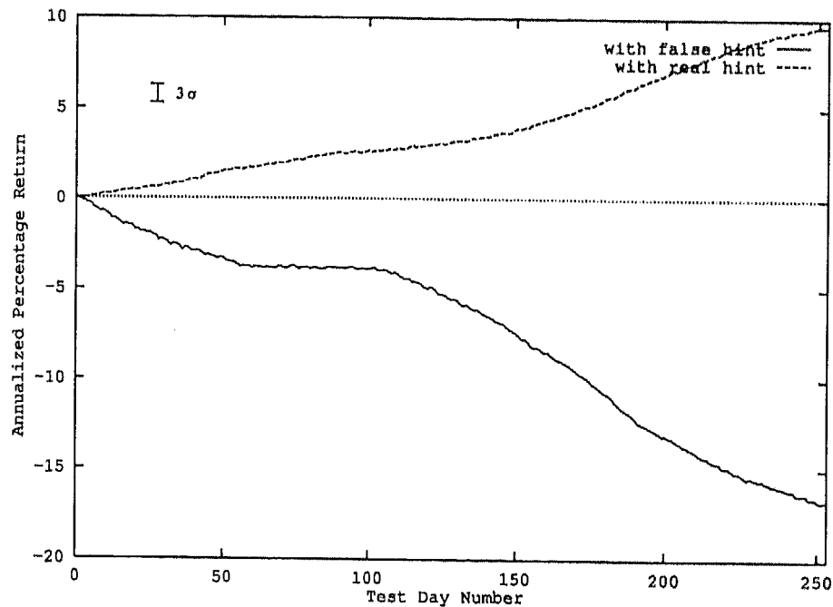
Figure 5. Performance of the real hint versus a false hint.
